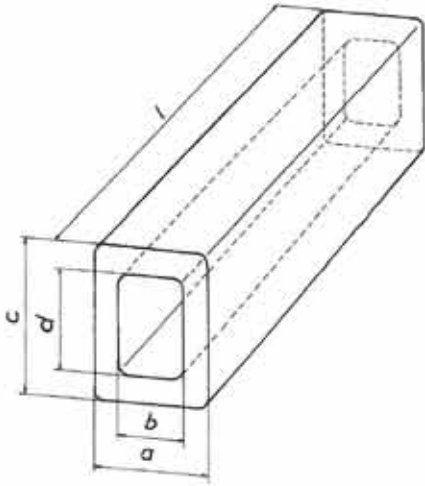
hollowbeam
